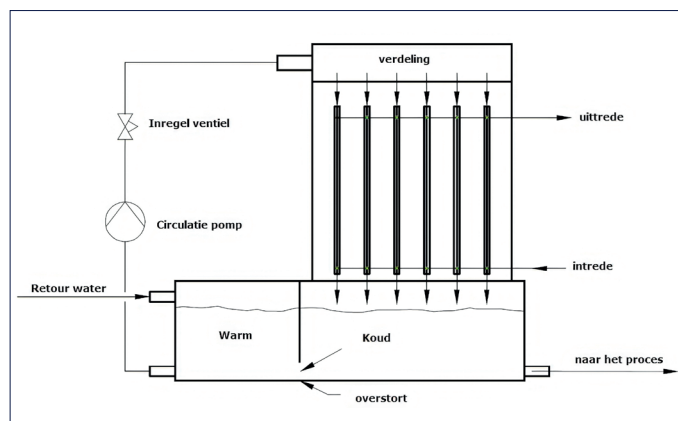
Fig. 2: Falling film-systeem (Buco HTT).
